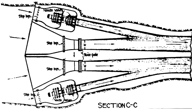
Fig. 51. Gates for controlling the small floods and the stored water supply for the proposed Dublin dam.
